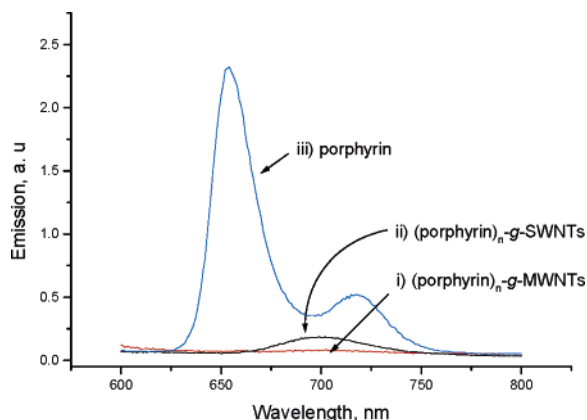
Figure 2. Steady-state fluorescence of (i) (por) n -g-MWNTs, (ii) (por) n -g-SWNTs, and (iii) por-OH in CHCl 3 at λ ex = 550 nm. The Soret band absorbance of [por] abs = 0.183, [(por) n -g-MWNTs] abs = 0.183, and [(por) n -g-SWNTs] abs = 0.364.
